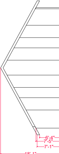
SECTION DD'
